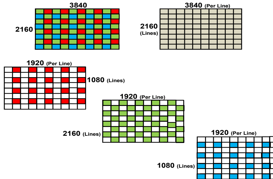
Figure 2 Illustrating the separate CFA array and the CMOS imager while also showing the CFA separated into its component color filters to better expose the structure of their respective sampling lattices
