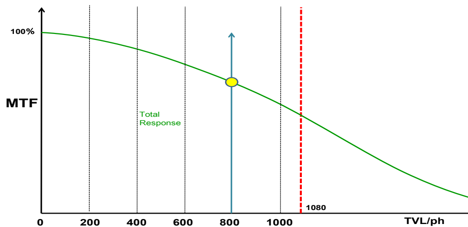
Figure 7 Showing the final horizontal MTF characteristic of the final green video
